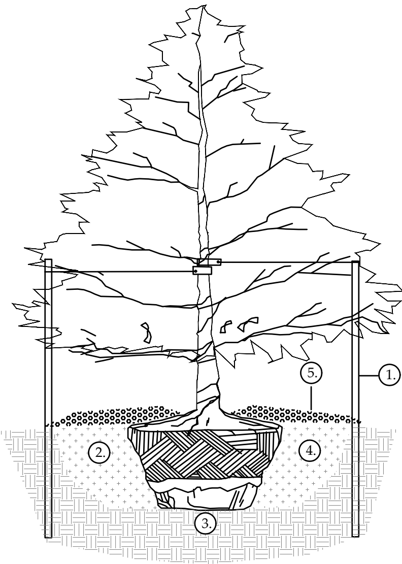
STAKING DETAIL
